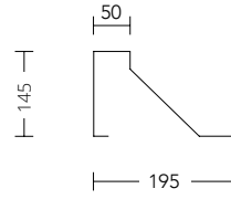
Section of roof stand
