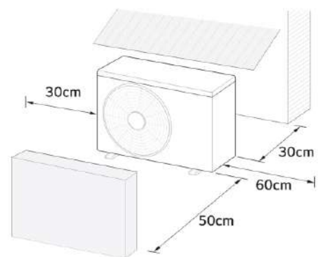
Outdoor Unit
