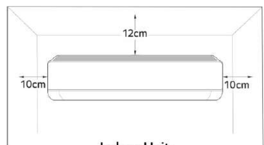
Indoor Unit
