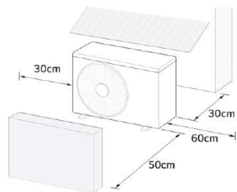
Outdoor Unit
