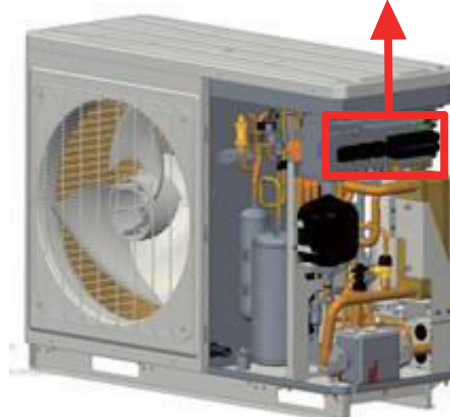
Terminal block XT5
