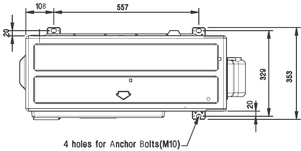
4 holes for Anchor Bolts(M10)
