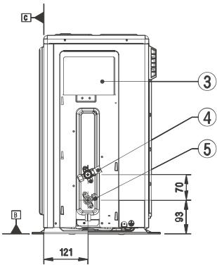
Side View (removed valve cover)
