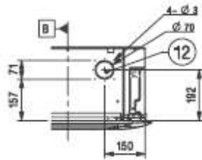
View A Fresh Air Intake hole
