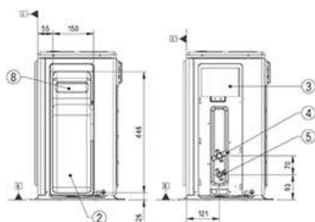
Side View (removed valve cover)
